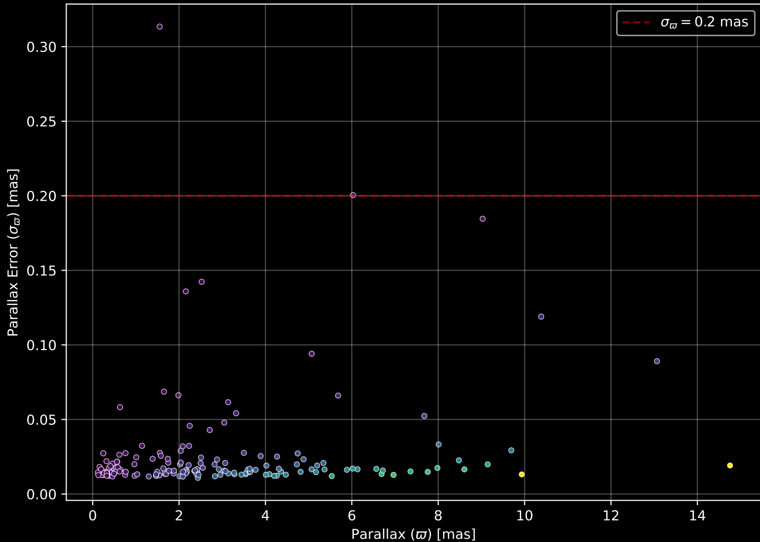
APOGEE DR17 Field: [033+43_MGA] Parallax Quality (n= 164)
