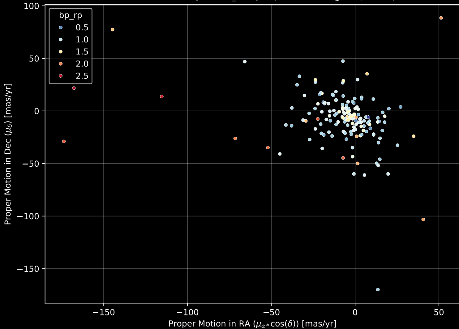
APOGEE DR17 Field: [033+43_MGA] Proper Motion Diagram (n= 164)
