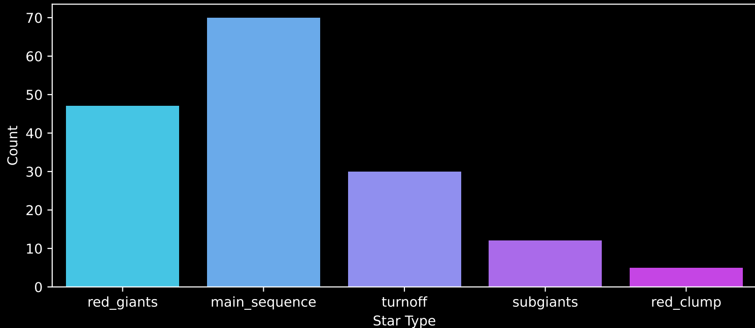
APOGEE DR17 Field: [033+43_MGA] Count plot of Star Type
