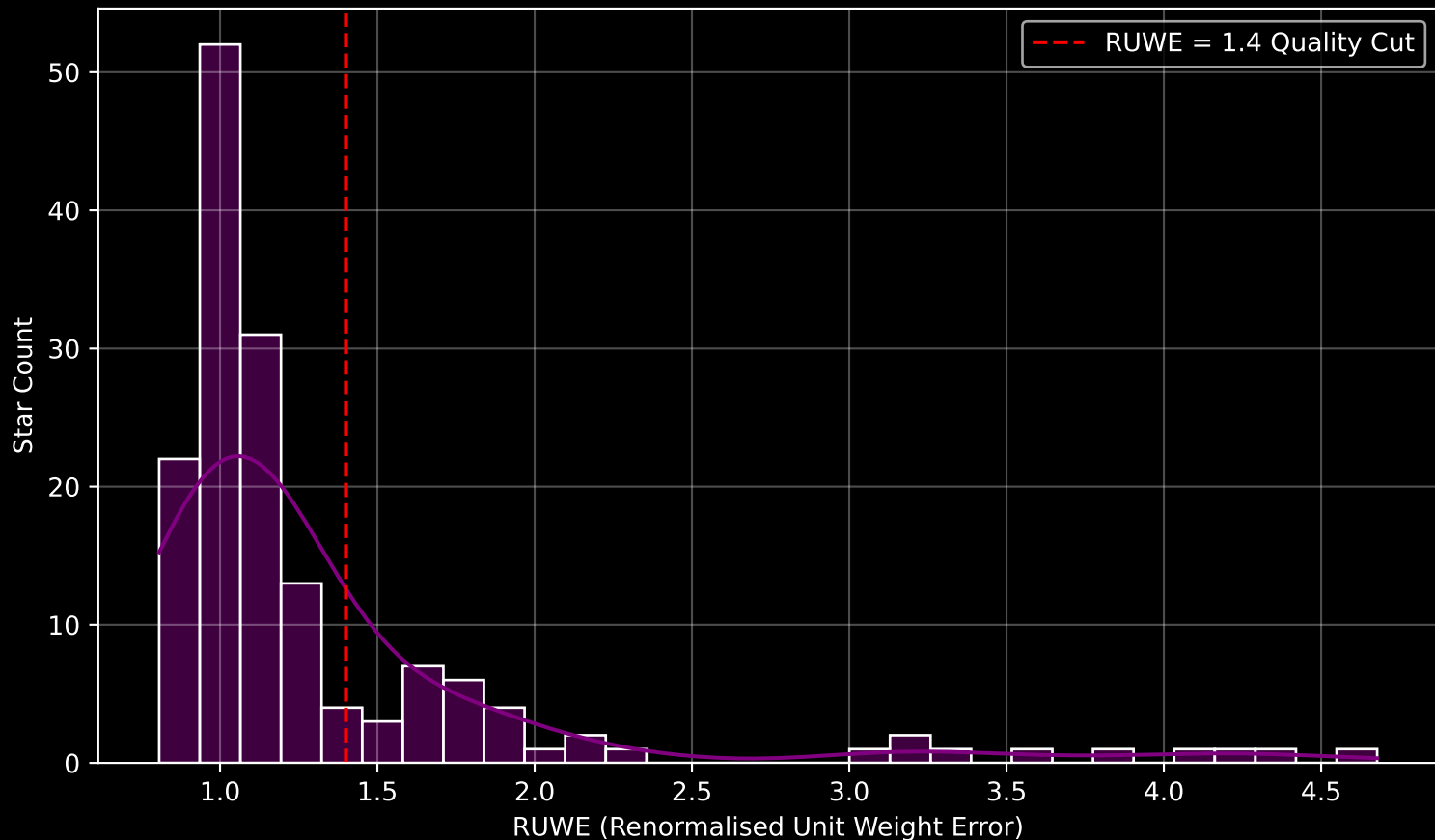
GAPOGEE DR17 Field [033+43_MGA] RUWE Distribution (n= 156)
