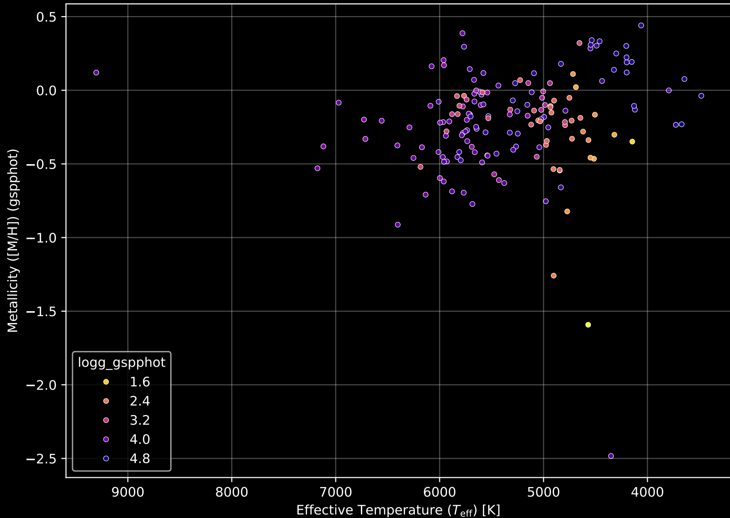
APOGEE DR17 Field: [033+43_MGA] Stellar Population Parameters (n= 164)
