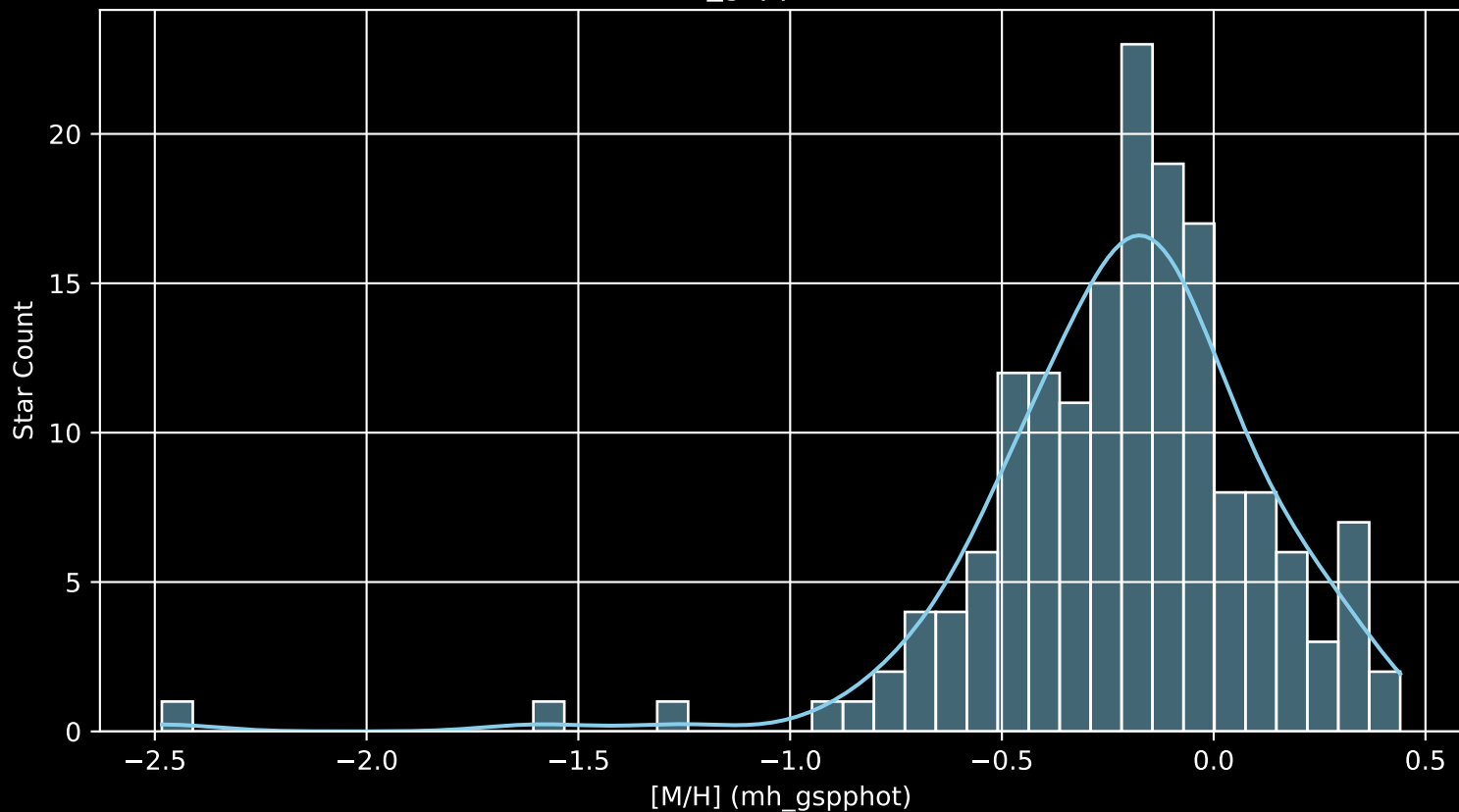
APOGEE DR17 Field: [033+43_MGA [M/H] (mh_gspphot) (n= 164)
